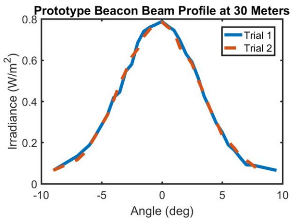
Figure 4. The irradiance profile of the prototype beacon's beam, measured from a distance of 30 meters.
