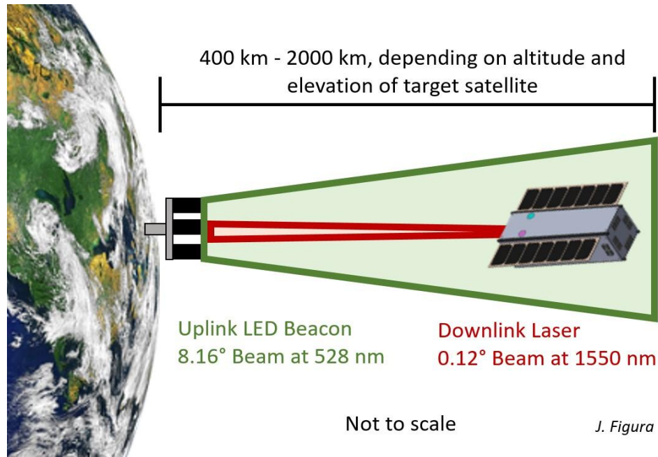
Figure 1. The concept of operations of the LED beacon, illustrating its use as part of a satellite laser communication system. The LED beacon's beam is shown in green and the downlink laser in red, coincident with each other.
