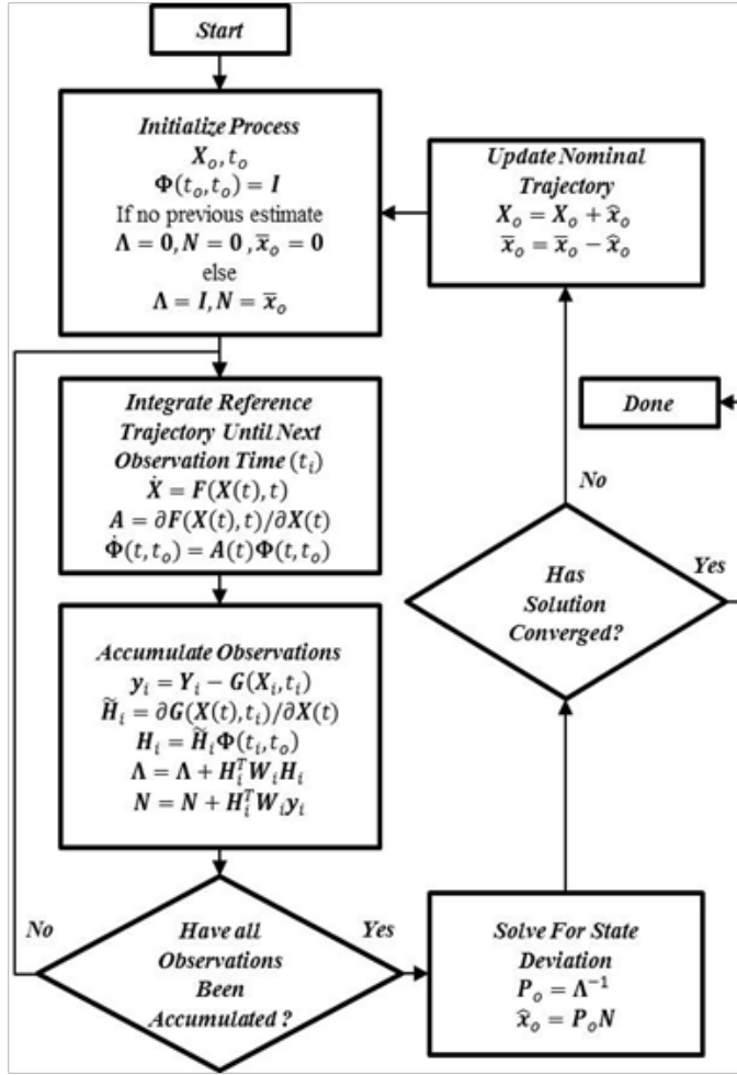
Figure 7. Batch Post-Processing Algorithm.
