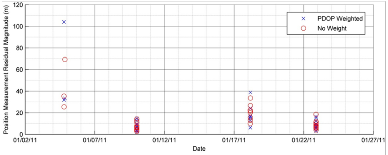
Figure 8. Position Measurement Residuals from Batch Post-Processing Algorithm Using Position Fixes As Measurements.
