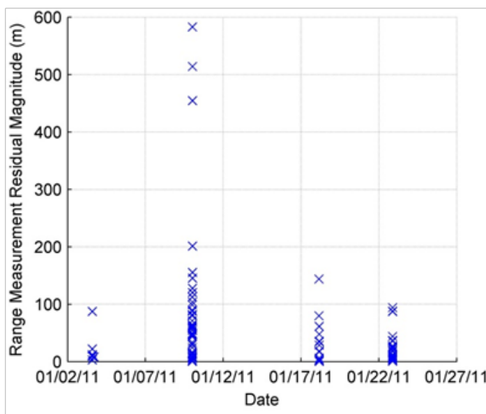
Figure 11. Range Measurement Residuals from Batch Post-Processing Algorithm Using Pseudo Range Measurements.
