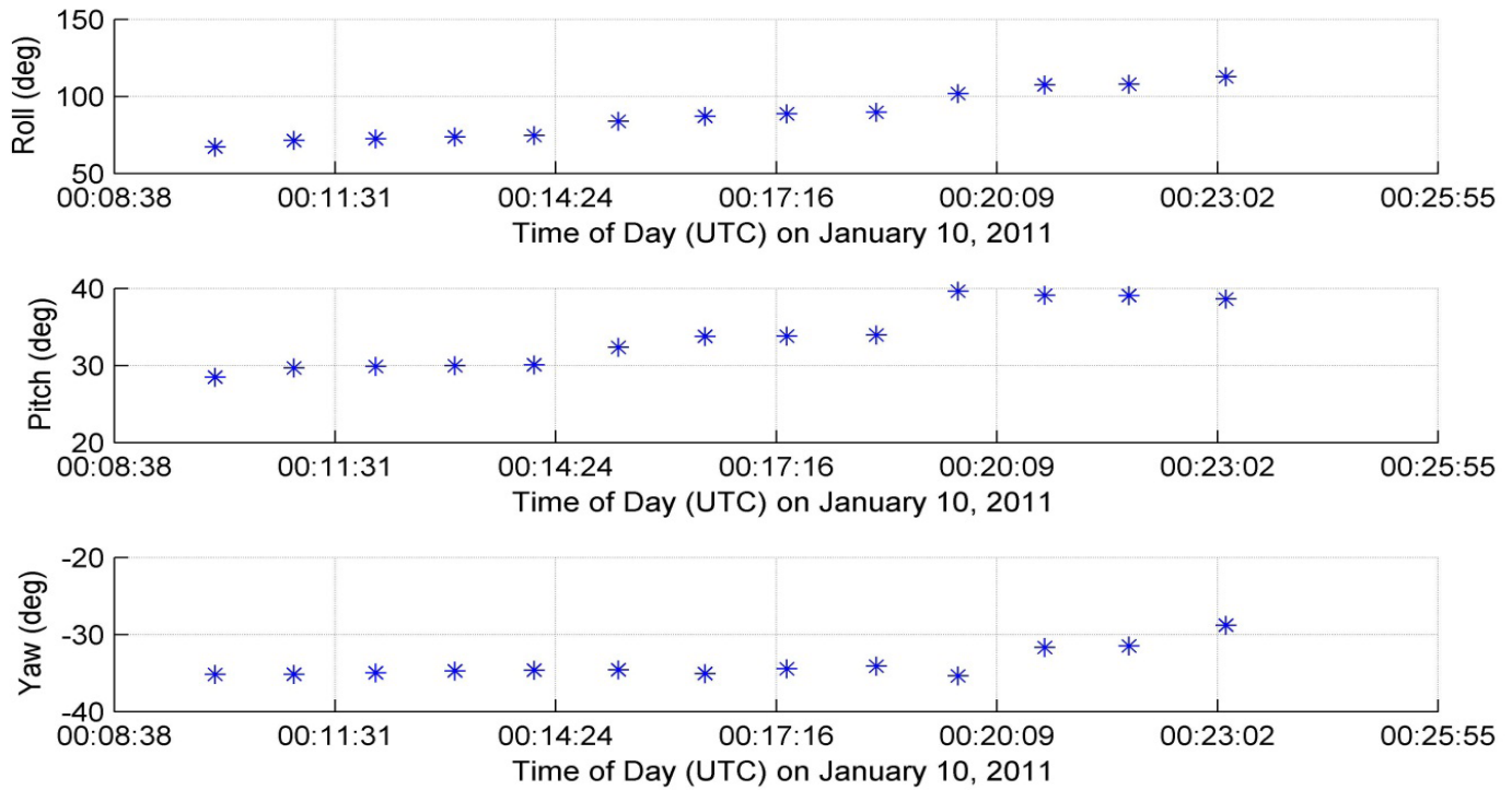
Figure 12. Reported GPS Receiver Attitude Solutions from January 10, 2011.
