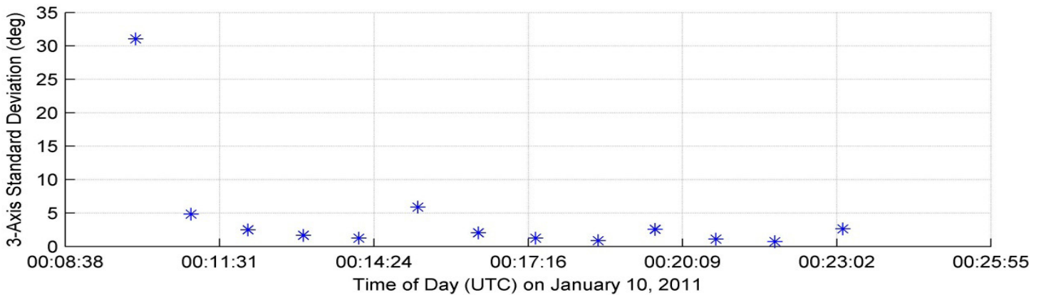
Figure 13. Reported Attitude Solution 3-Axis Standard Deviation from January 10, 2011.
