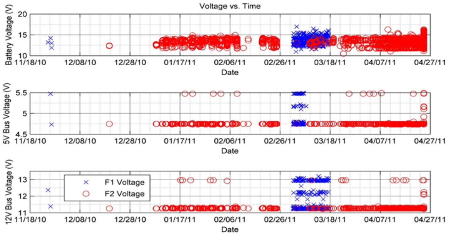
Figure 3. Voltage Bus Levels on FASTRAC Satellites.
