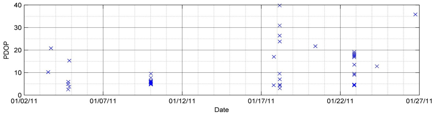
Figure 6. Reported PDOP from downloaded GPS messages showing on-orbit position fixes.
