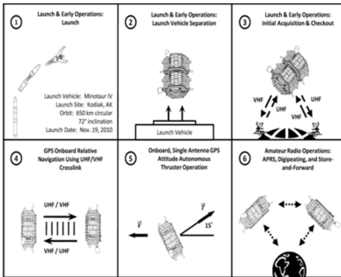
Figure 2. FASTRAC Concept of Operations.
